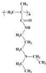
Figure 1. Structure of poly( N -[3-(diethylamino)propyl]methacrylamide)
