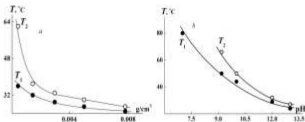
Figure 2. Dependences of temperatures T_1 and T_2 on (a) concentration at pH 13 and (b) acidity of medium at c = 0.008 g/cm^3 for PDEAPMA buffer solutions.
