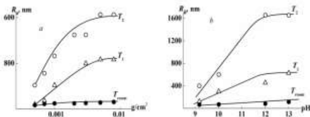
Figure 2. Dependences of temperatures T_1 and T_2 on (a) concentration at pH 13 and (b) acidity of medium at c = 0.008 g/cm^3 for PDEAPMA buffer solutions.
