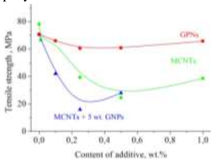
Figure 3. – Dependence of the tensile strength vs. concentration of additives for the epoxy based composites filled by different amount of MCNTs, GNPs, and MCNTs/GNPs
