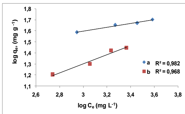
Figure 2: Freundlich, adsorption isotherm, (a) Ca 2+ and (b) Mg 2+ (T=313 K)
